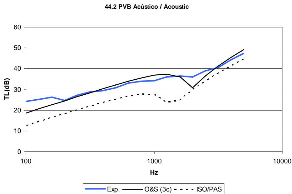
Figure 1: Prediction models without layer coupling. Ookura-Saito for three layers and ISO/PAS 16940:2004 with global parameters [7].
