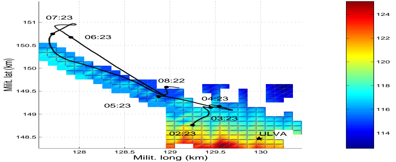
Figure 1: INTIFANTE'00 Event I source-receiver geometry and bathymetry; ULVA refers to the VLA position.
