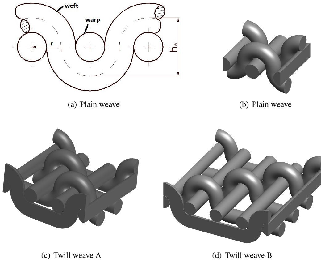
Figure 1: Cross-sectional drawing and simplified 3D models
