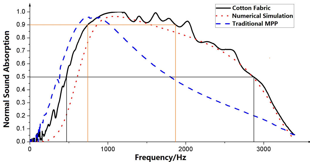
Figure 4: Comparison of optimized woven fabric and traditional MPP with the depth of air cavity D=50\text{mm}
