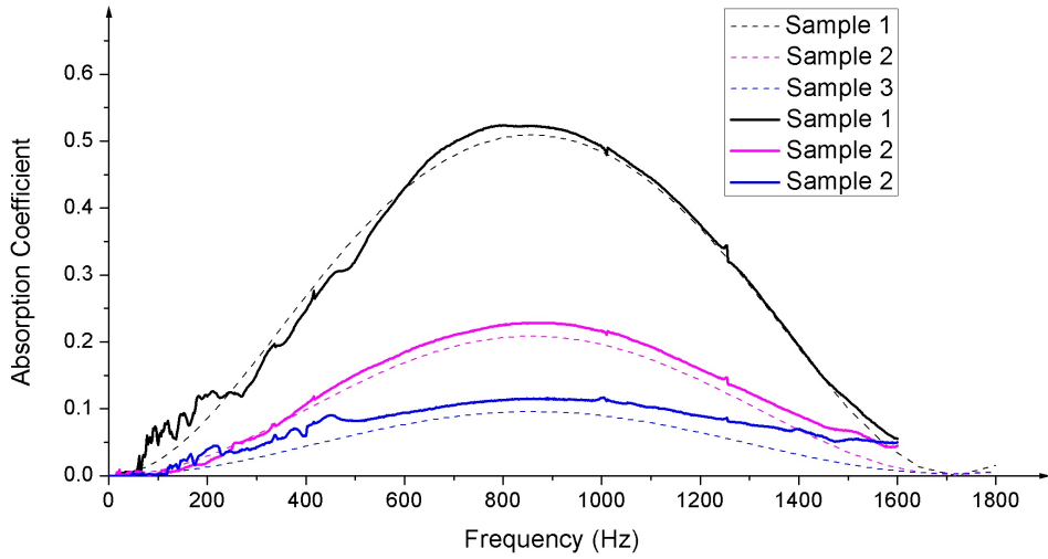
Figure 2: The results of numerical simulation method and experiments of sample 1, 2, 3 with the depth of air cavity D=100\text{mm}
