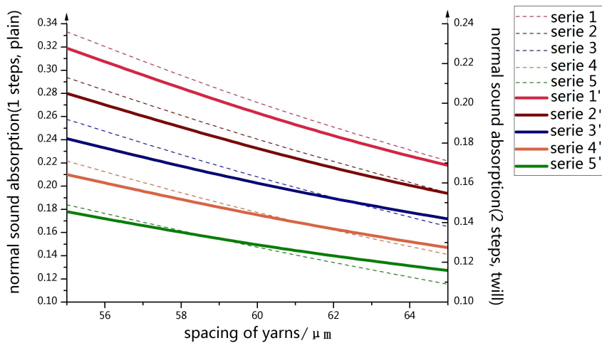
Figure 3: The peak values of sound absorption curve of all samples(full lines are plain weave results, dotted lines are twill weave results)
