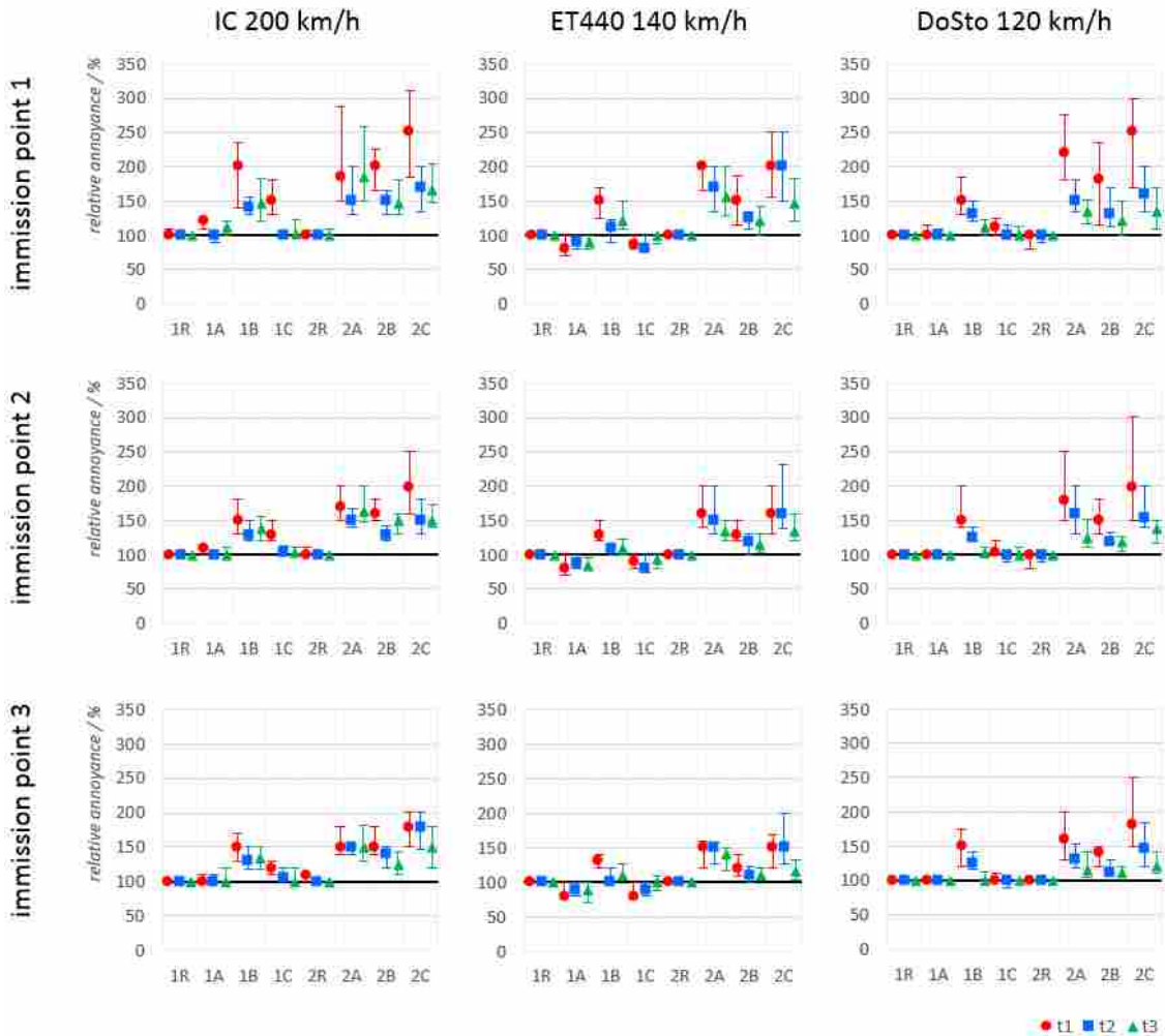
Figure 3: Annoyance caused by trains passing after the grinding process on the respective grinding section. Upper graphs: point of immission 1 (garden in front of the house), middle graphs: point of immission 2 (living room with tilted windows), lower graphs: point of immission 3 (living room with closed windows). Red: t1 (zero loading tons), blue: t2 (700k loading tons), green: t3 (1mio loading tons).
