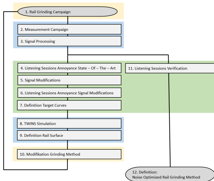
Figure 1: Overall concept of the project “Noise optimized rail grinding” of DB Netz AG Yellow: DB Netz AG, blue: DB Systemtechnik, green: Möhler + Partner Ingenieure AG
