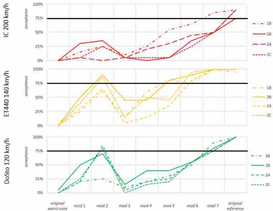
Figure 5: Threshold of acceptance for the different kind of trains
