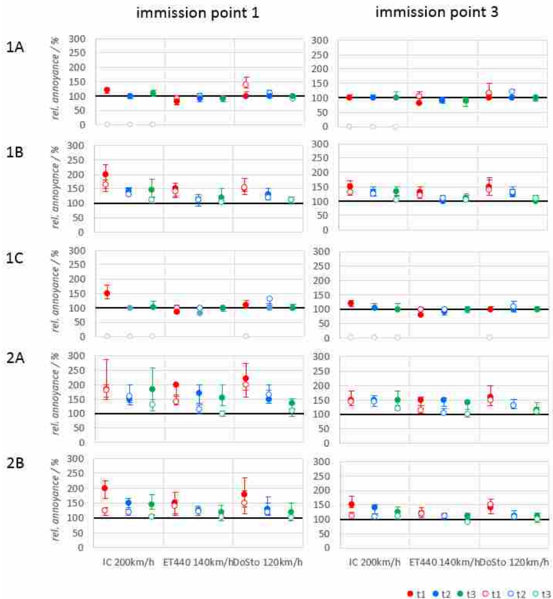
Figure 6: State-of-the-art (filled symbols) versus validation (open symbols).
