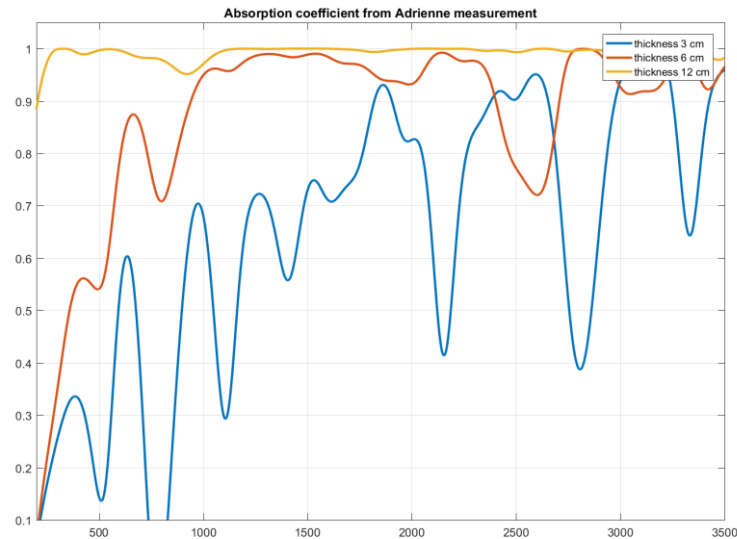
Figure 5 – Absorption coefficient from Adrienne measurement.
