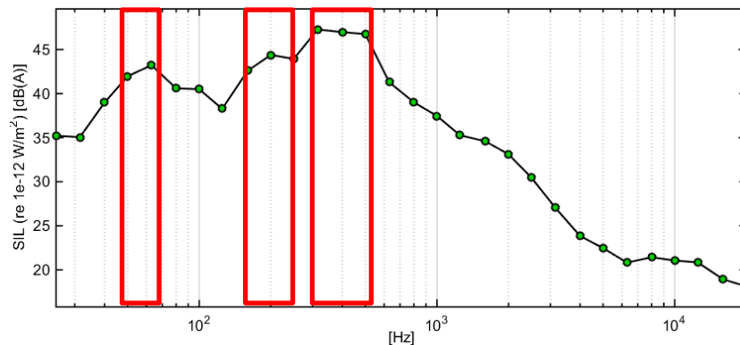
Figure 9. A-weighted power spectrum of the active intensity in 1/3 octave bands with the car idling at 3000 rpm.
