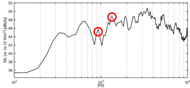
Figure 12. A-weighted power spectrum of the active intensity. The red circles indicate two resonances, which are visualized in Figure 13.
