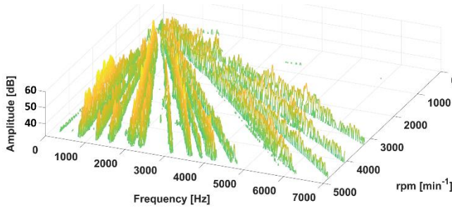
Figure 5: Logarithmically scaled amplitude magnitudes of the run-up signal in dependency of its variables, rotational speed and frequency.
