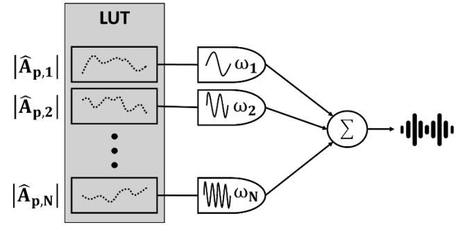
Figure 7: Block diagram of the synthesis step by superposition of N discretized amplitude magnitudes (left) and N sinusoidal oscillators (right).
