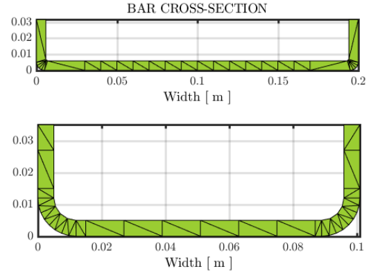
Figure 2: Cross section of the aluminium bars considered in this work for the lowest tones (top) and highest tones (bottom).
