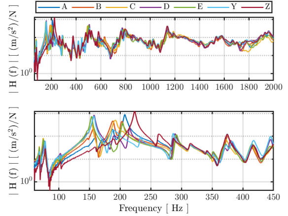
Figure 7: Magnitude of the measured transfer functions as the location of the soundpost is varied. Input acceleration measured close to the bridge.
