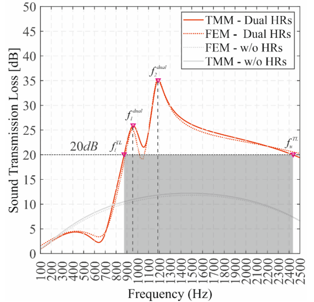
Figure 6. Evaluation of the nSTL for a dual symmetric proposition for two different frequencies f_1 = 950\text{ Hz} and f_2 = 1200\text{ Hz} . The solid lines represent the TMM results, and the dotted lines the numerical results, respectively.
