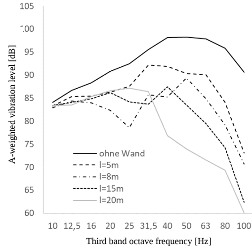
Figure 5: Frequency analyses for the distance of 50m.
