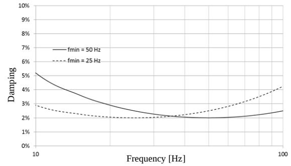
Figure 3: Rayleigh damping f_{\min} from 50Hz to 25Hz.
