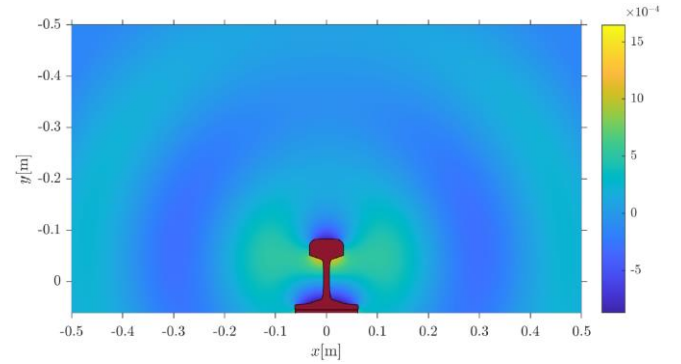
Figure 4. Radiated noise for a load acting at the midpoint of the railhead at a frequency of 1000 Hz .
