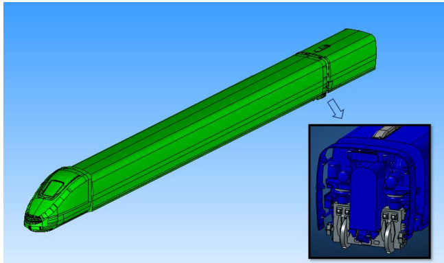
Figure 2. Geometry used to model the airflow in the inter-coach gap.
