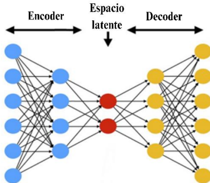
Figura 4. Autoencoder Fully-connected.
